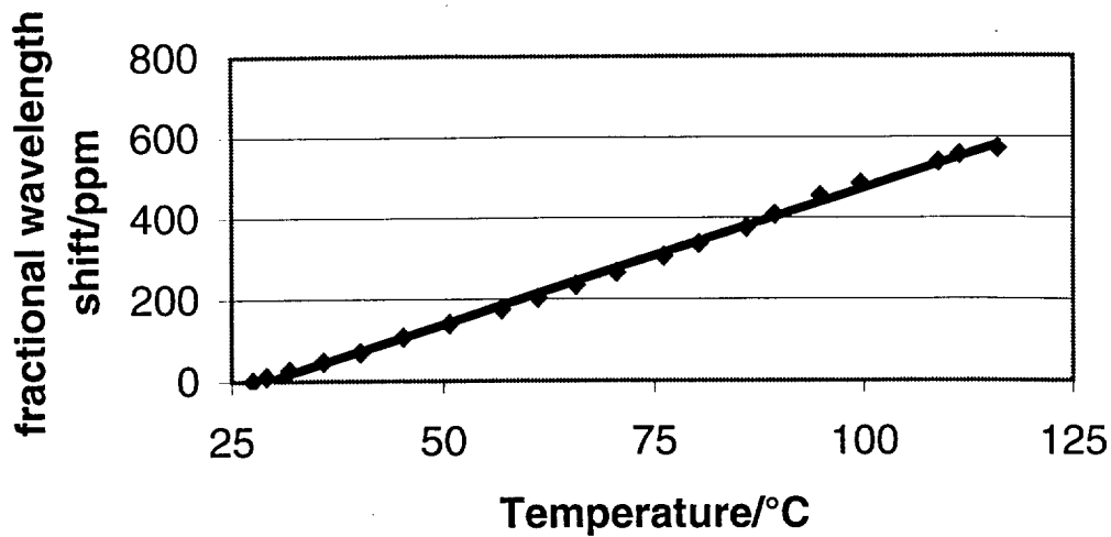
Figure 4b. Response of the same sensor to temperature under constant load.
