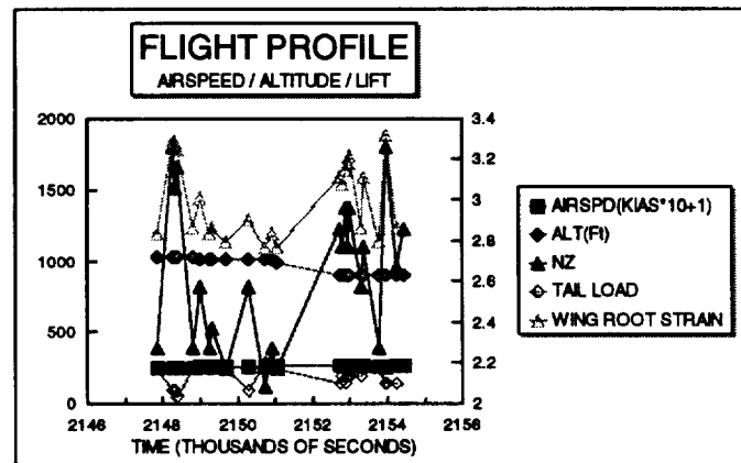
Figure 1b Zoom on Figure 1a Overstress Incident
