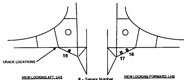
FIGURE 10. WHEEL WELL RADIUS SENSOR LOCATIONS.
