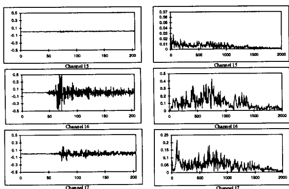
FIGURE 12. CRACK GROWTH EVENT.
