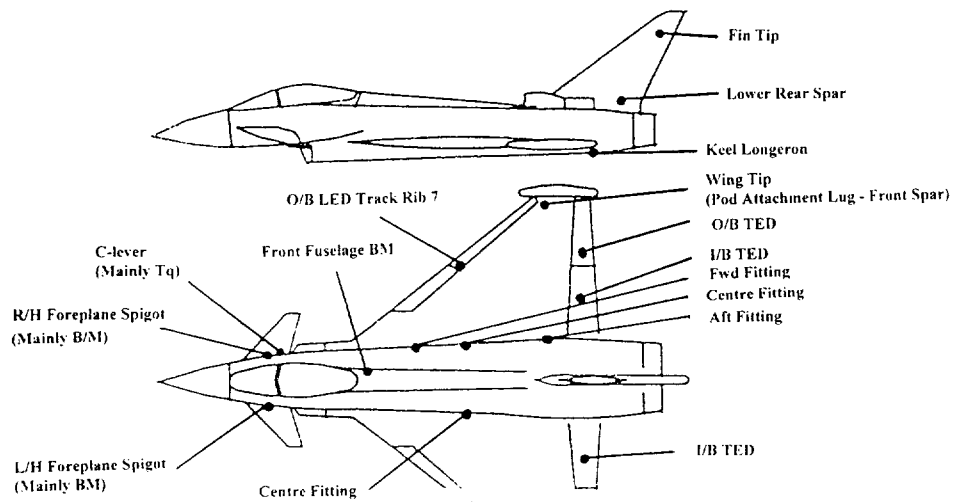
FIGURE 4A - SHM MONITORED LOCATIONS - BASELINE FIT
