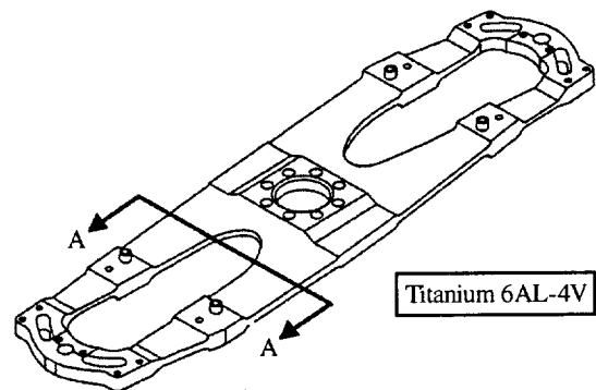
Figure 2.4 Main Rotor Yoke Geometry
