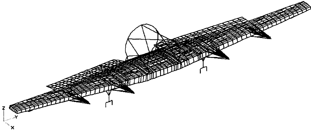
Figure 3 Wing Finite Element Model
