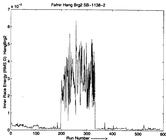
Fig. 22. Hanger Bearing Inner Race Energy.
