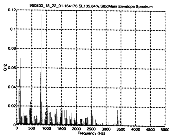
Fig. 34. Fault Spectrum for Bearing SB 3313.
