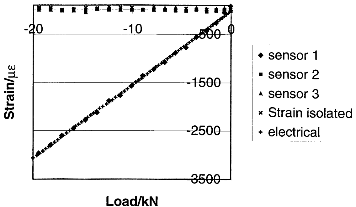
Figure 4c. Combined sensor response for all sensors in the optical rosette strain gauge. The loading direction is parallel to sensor 1 (constant temperature).
