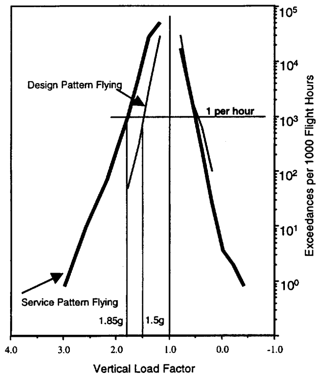
Figure 6 - Wings Forward Load Factors
