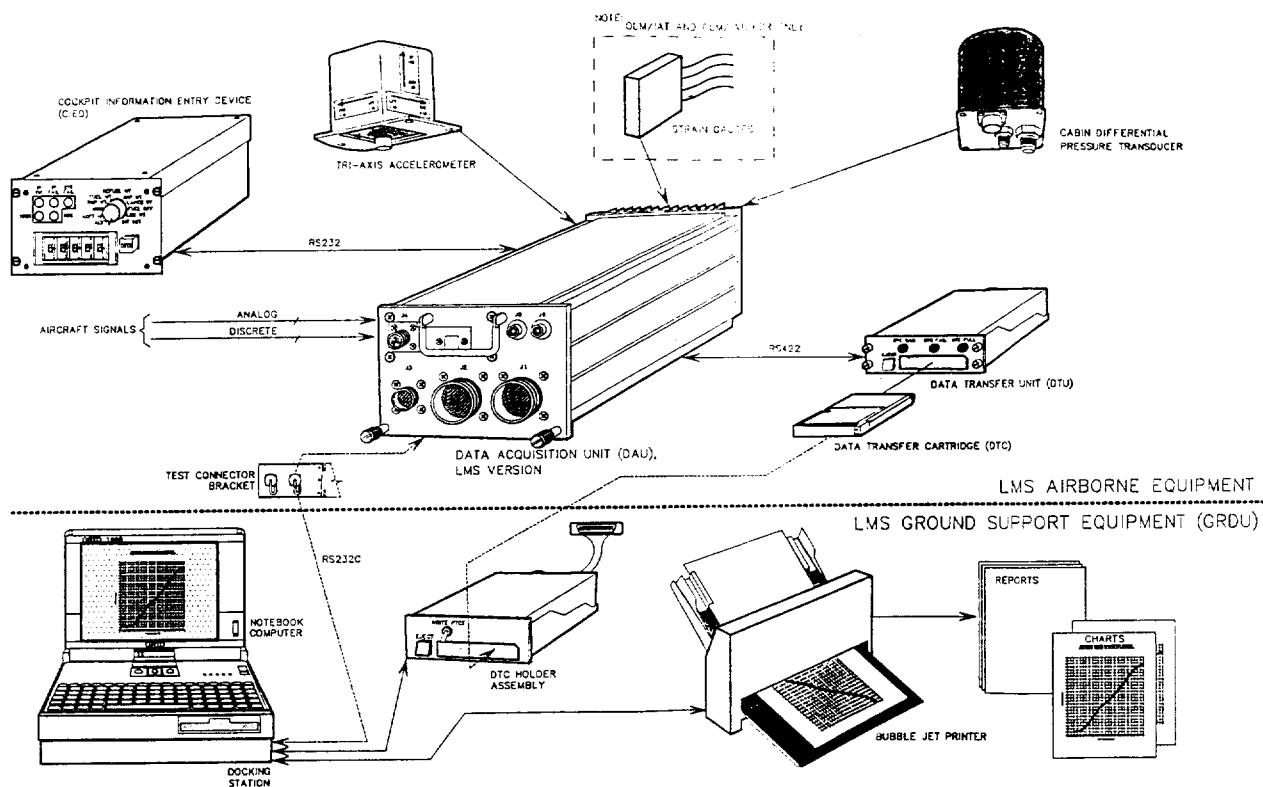
Figure 14.1 OLM/IAT System Components
