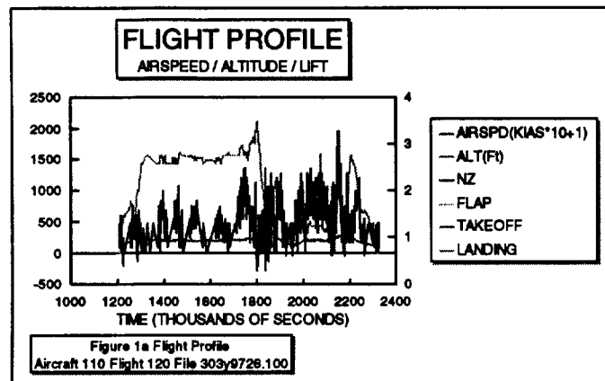
Figure 1a Flight Profile of an Overstress Incident
