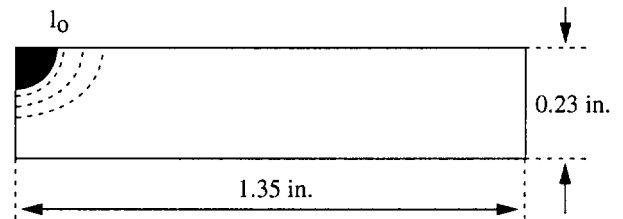
Figure 4.2 Collective Lever Section A-A
