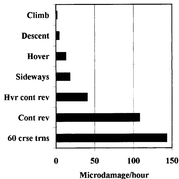
Figure 8 Microdamage/hour - 50% cumulative probability
