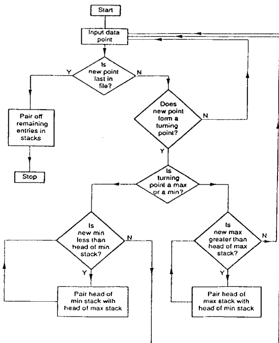
Figure 3. Basic structure of Rainflow sub-routine.
