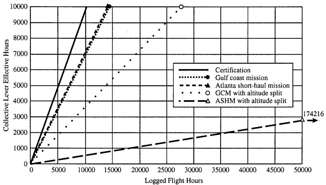
Figure 3.3 Effective Usage Collective Lever
