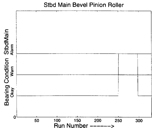
Fig. 26. SB 2205 Condition Call from Starboard Sensor.
