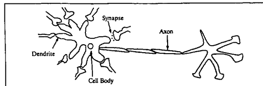
Biological neuron
