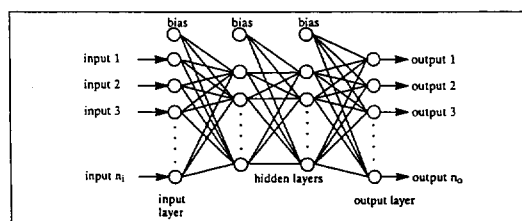
Neural Network
