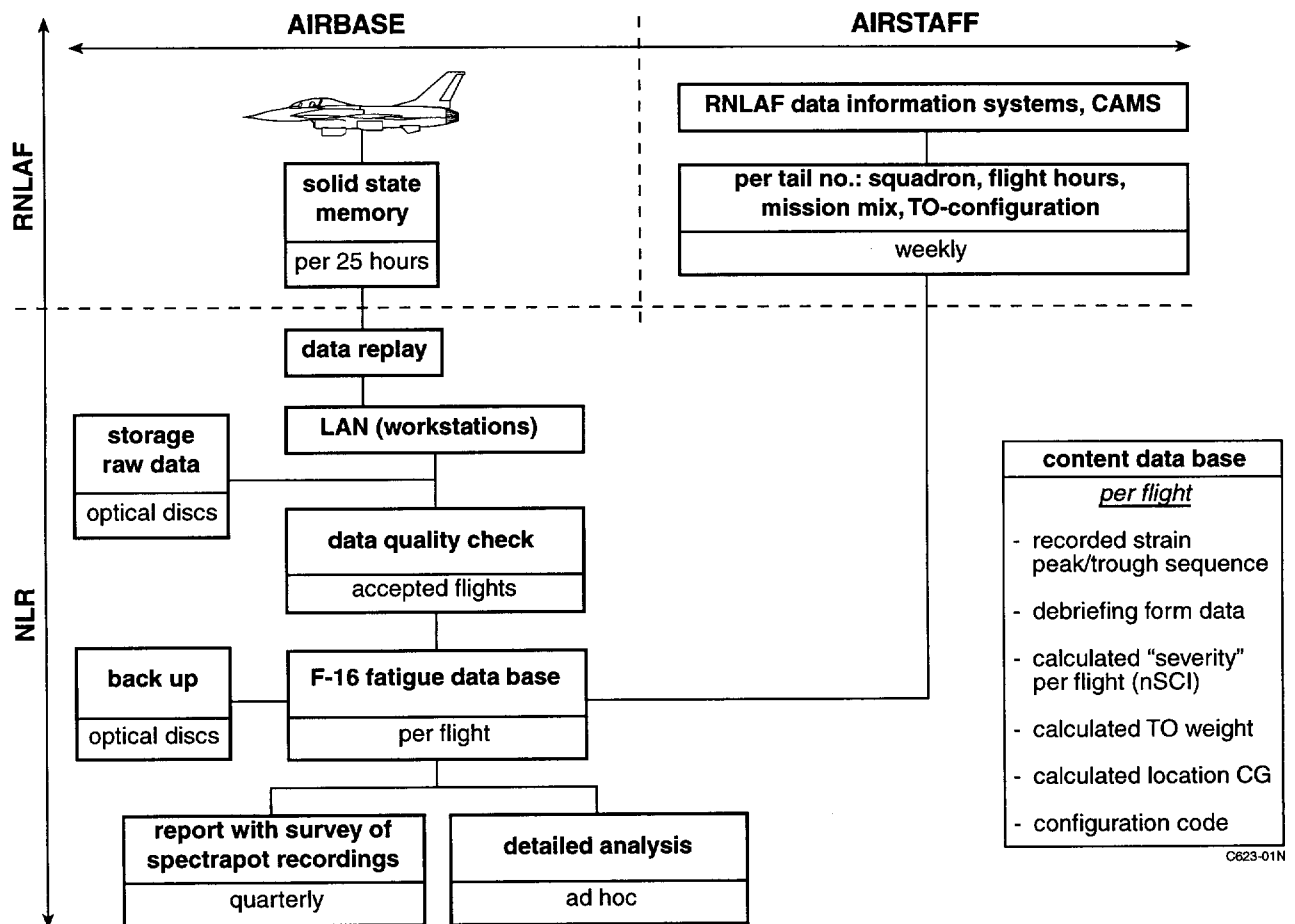
Fig. 1 Data flow in F-16 load monitoring program
