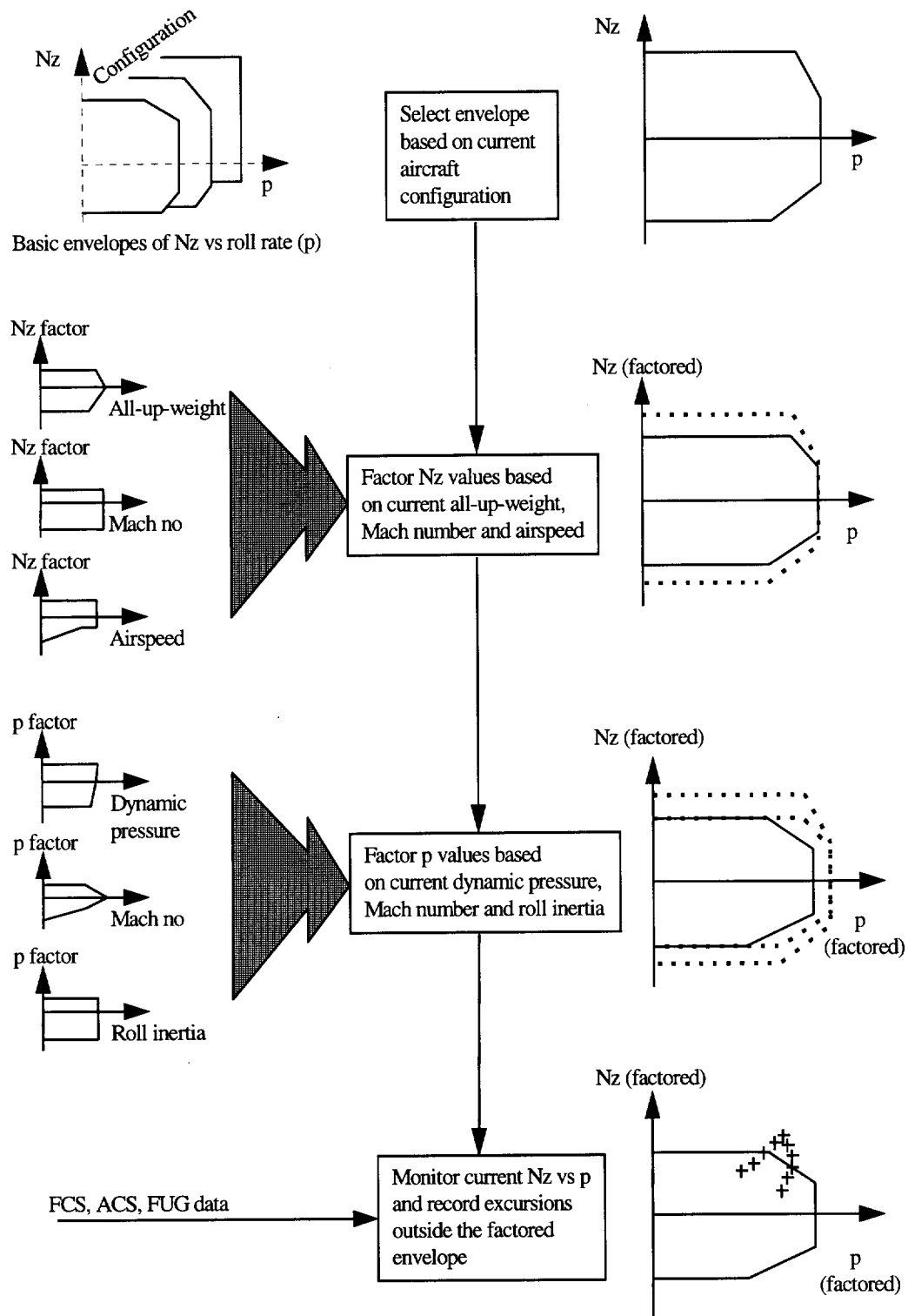
Figure 5 Example of Structural Event Monitoring
