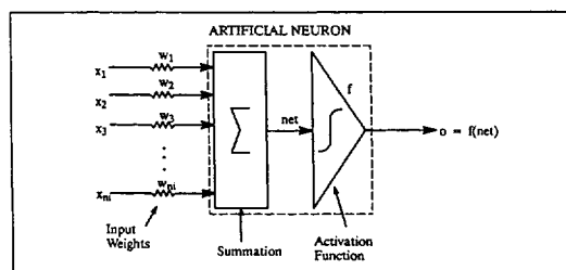
Artificial Neuron
