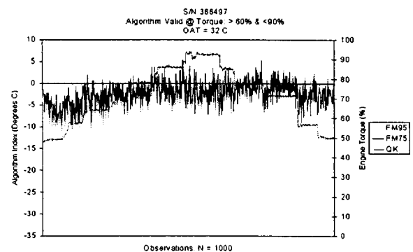
Fig. 18. T700 Engine Algorithm Results.
