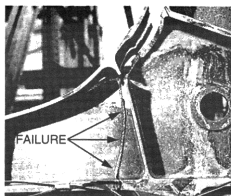
FIGURE 10. CATASTROPHIC FATIGUE FAILURE OF BULKHEAD
