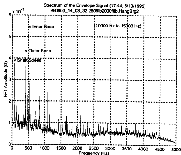
Fig. 21. Rejected Hanger Bearing Spectral Plot.
