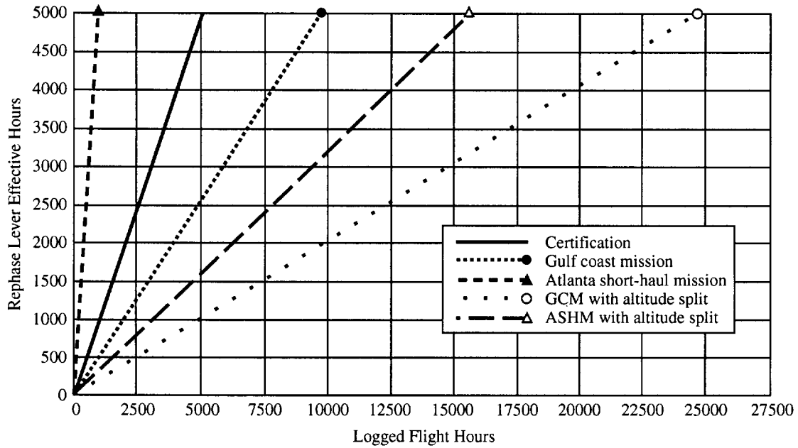
Figure 3.2 Effective Usage Repphase Lever
