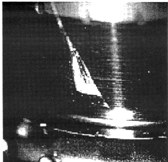
Fig. 16. Main Transmission Input Pinion Crack.
