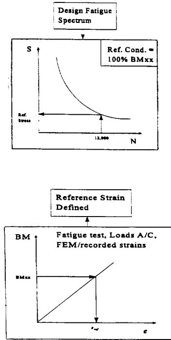
Figure 6 - Reference Stress/Strain
