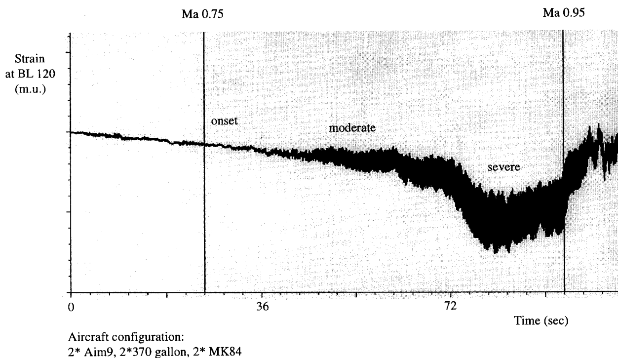
Fig. 10 Example of Limit Cycle Oscillation recording
