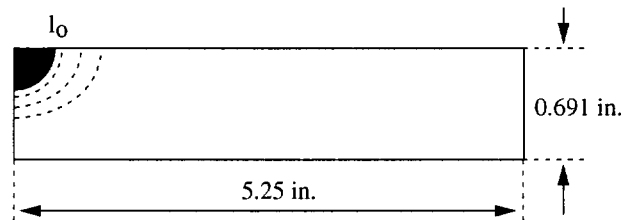
Figure 4.4 Main Rotor Yoke Section A-A
