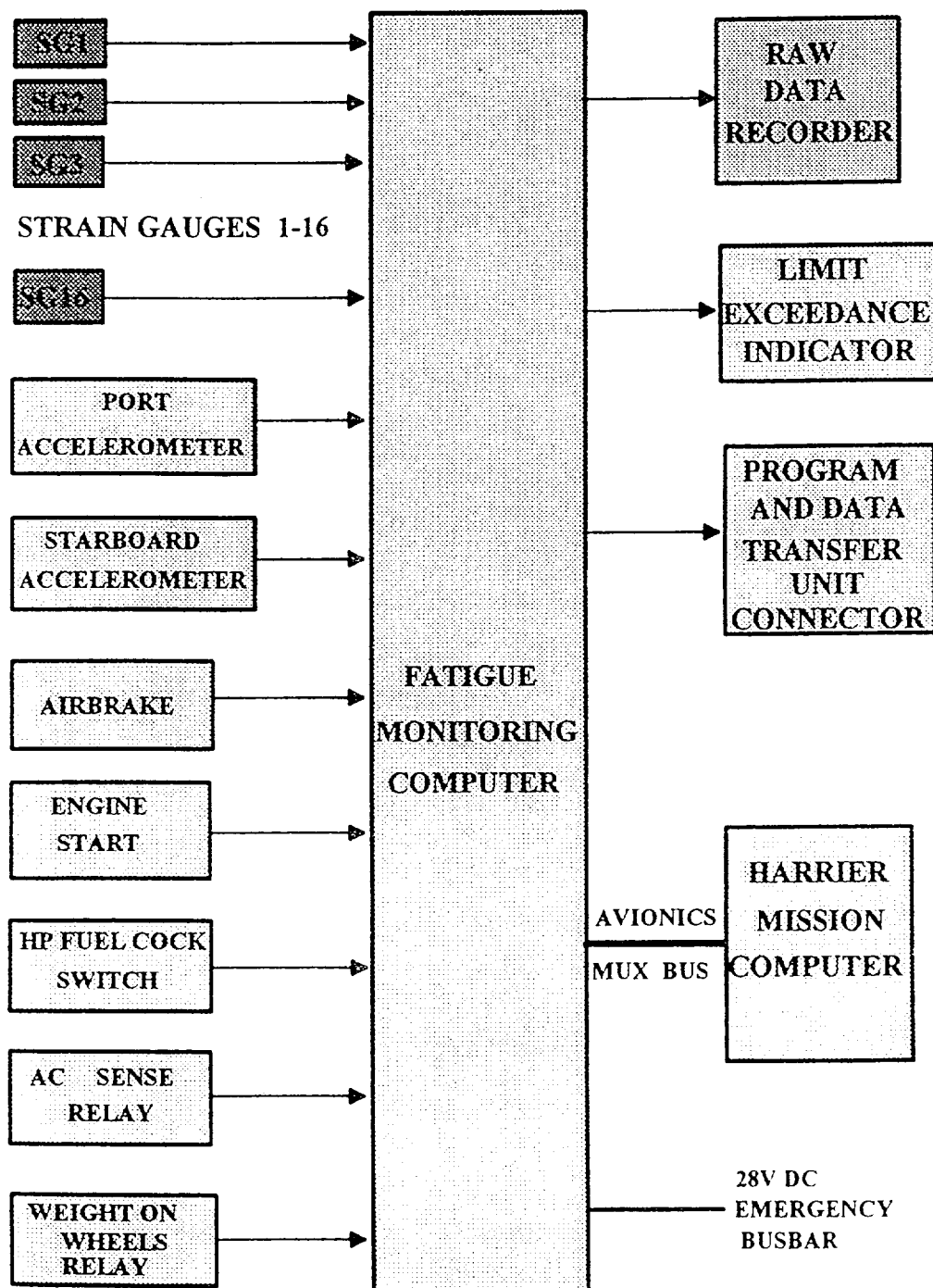
FIGURE 3B - FMCS SCHEMATIC
