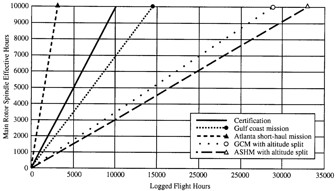
Figure 3.4 Effective Usage Main Rotor Spindle
