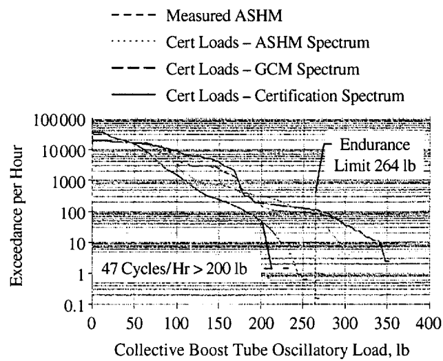
Figure 5.1 Collective Boost Tube Load Comparison
