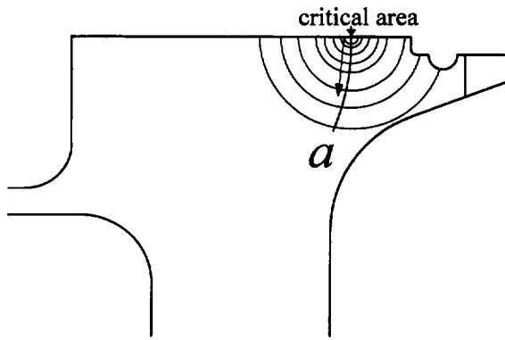
Figure 2: Analysed crack fronts and crack path a
