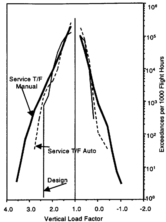
Figure 7 - Wings Aft Load Factor Data
