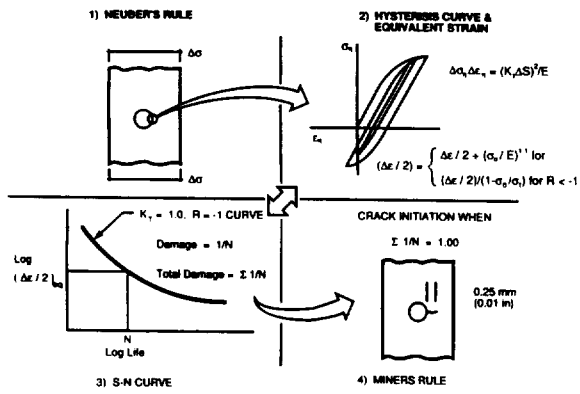
Figure 5 - Crack Initiation Concept
