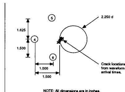
(b) Typical Source Location Results
