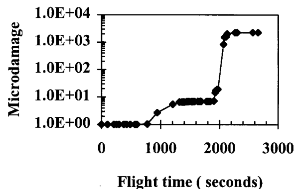
Figure 9 Cumulative damage throughout selected flight
