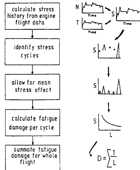
Figure 2. Procedure for calculating low cycle fatigue usage.
