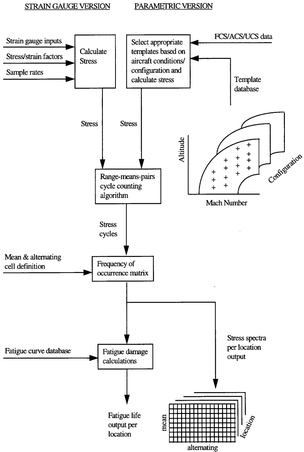
Figure 3 Overview of Fatigue Calculations
