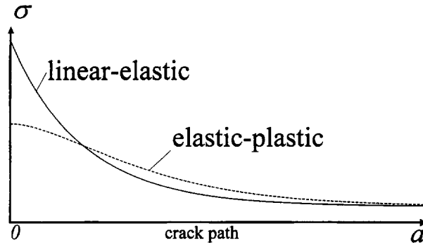
Figure 3: Stress redistribution due to plastification
