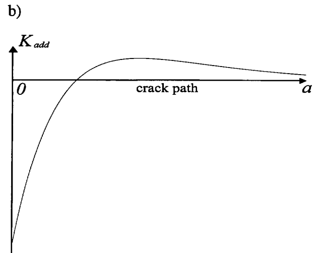
Figure 4: Geometry function g and additive term K_{\text{add}}
