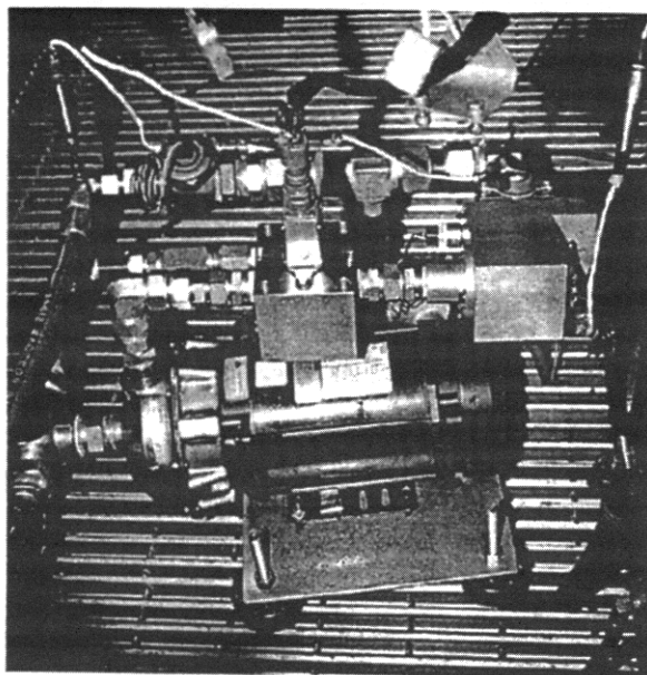
Fig. 32. Test Rig for Oil Monitoring Evaluation.
