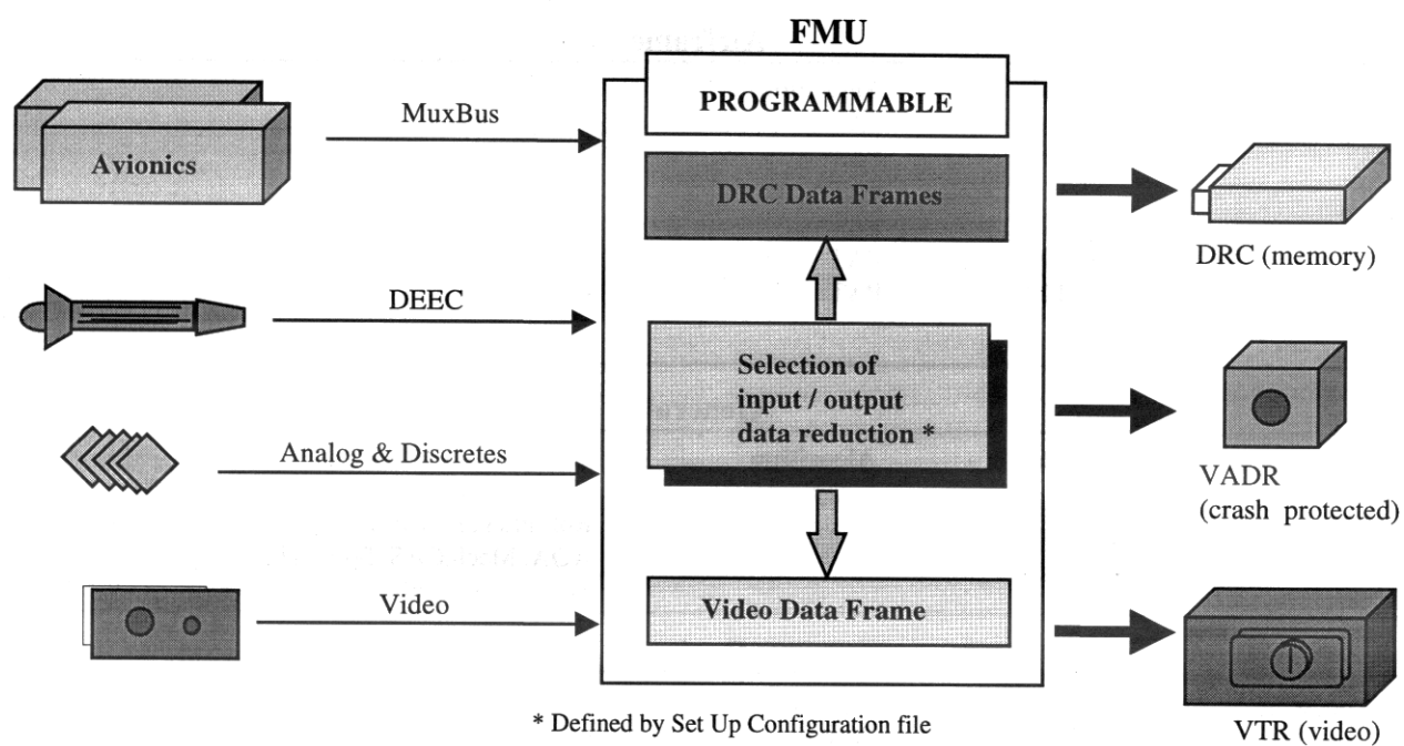
Fig. 7 Overview FACE system structure
