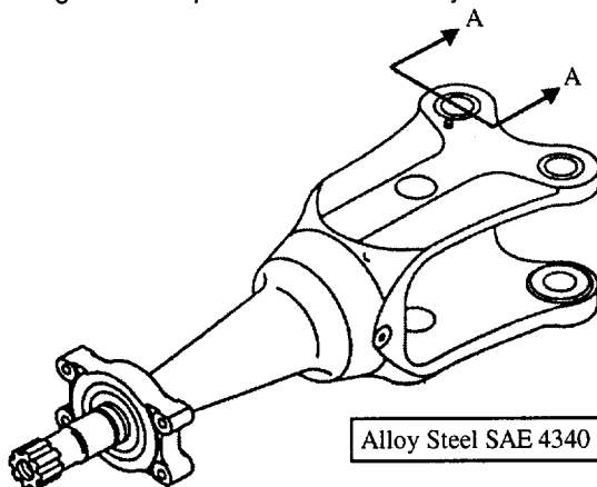
Figure 2.1 Rephase Lever Geometry
