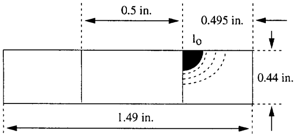
Figure 4.1 Rephase Lever Section A-A
