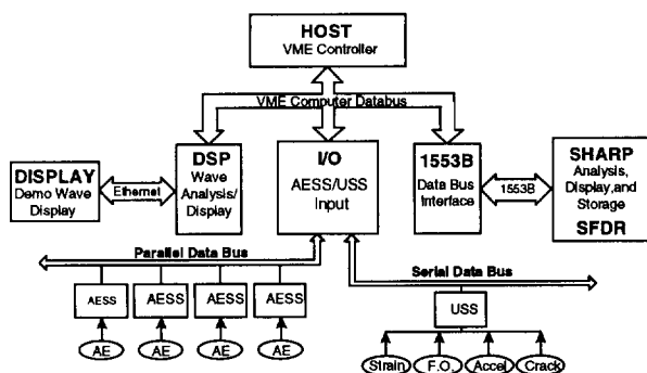
Figure 2. SHMS System Architecture
