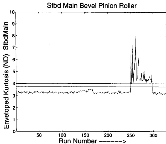
Fig. 28. SB 2205 Starboard Main Kurtosis Trend.
