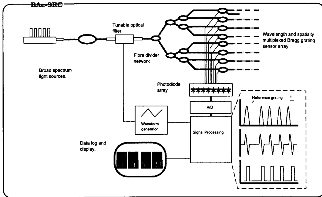
Figure 1. Optical strain sensor architecture based on in-fibre Bragg grating sensors.
