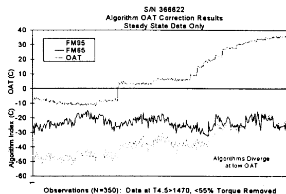
Fig. 19. Algorithm Correction Results.
