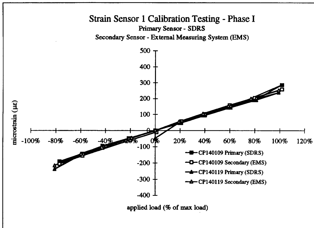
Figure 5a SDRS Calibration Phase I Test Results
