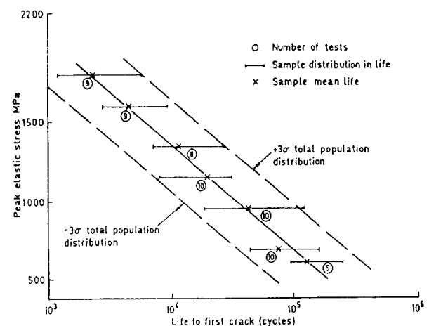
Figure 4. Notch fatigue data for Ti 6/4.
