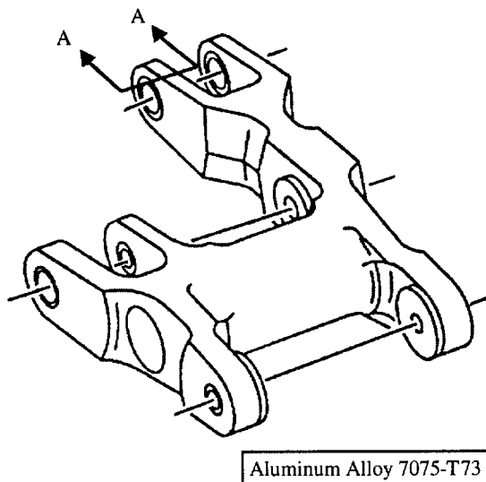
Figure 2.1 Rephase Lever Geometry
