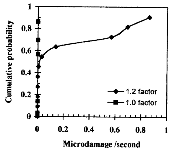
Figure 6 Hover - comparison of damage rate with loads factors of 1.2 and 1.0
