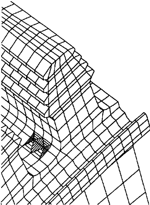
Figure 1: Remeshed FE model of a turbine disc in the vicinity of an introduced crack.
