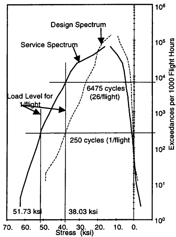
Figure 8 - Wing Carry Through Lower Cover Stress
