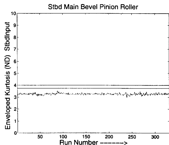
Fig. 31. SB 2205 Starboard Input Kurtosis Trend.
