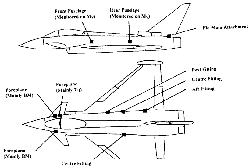
FIGURE 4A - SHM MONITORED LOCATIONS - BASELINE FIT
