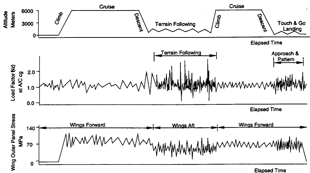
Figure 3 - Typical Mission Time History
