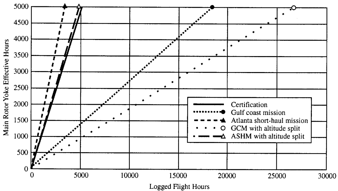
Figure 3.5 Effective Usage Main Rotor Yoke
